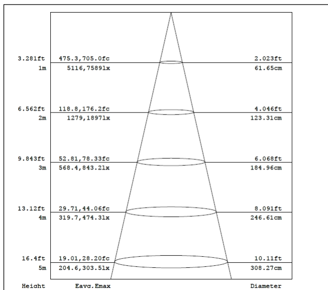
Diagram for RTM3540-xx in 4,000K. Other diagrams available on request
