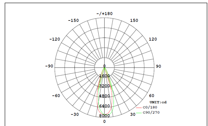
Diagram for RTM3540-xx in 4,000K. Other diagrams available on request
